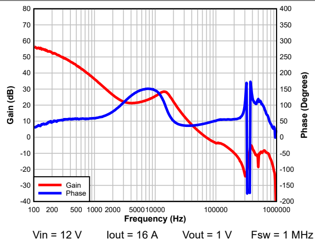
Figure 8-7. Bode Plot
