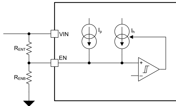
Figure 7-1. Adjustable UVLO Using EN
