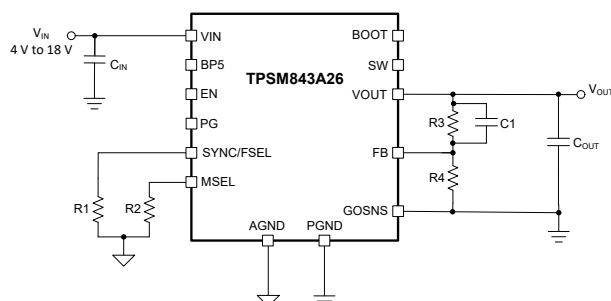
TPSM843A26 Simplified Application
