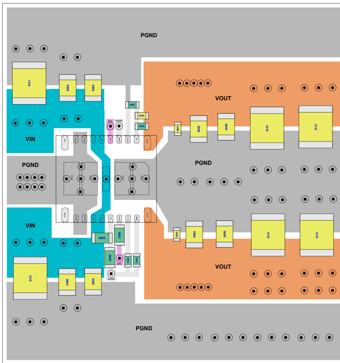
Figure 8-17. Example PCB Layout
