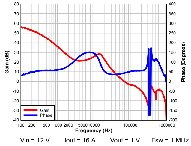
Figure 8-7. Bode Plot
