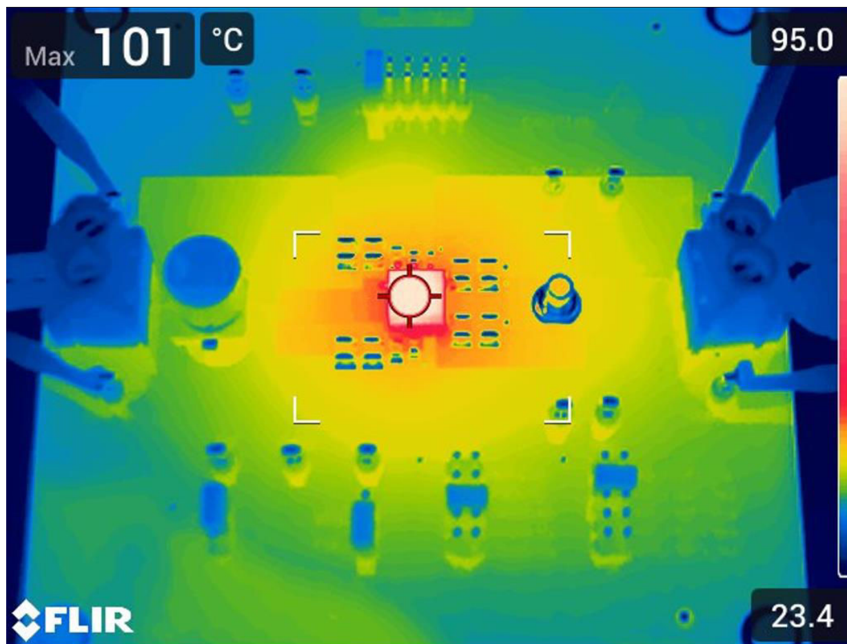
Figure 8-18. Thermal Image at 25^{\circ}\text{C} Ambient
