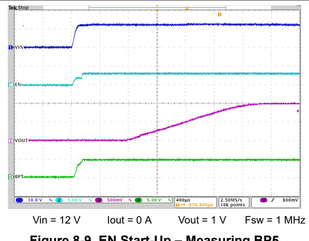
Figure 8-9. EN Start-Up – Measuring BP5
