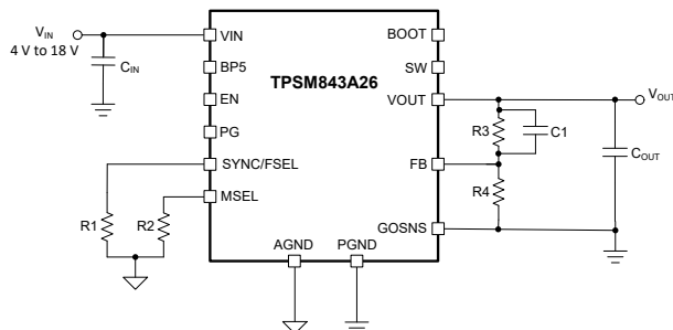
TPSM843A26E Simplified Application
