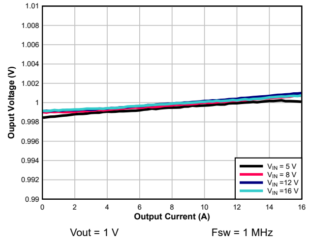
Figure 8-5. Load Regulation
