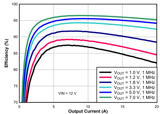
Typical Application Efficiency
