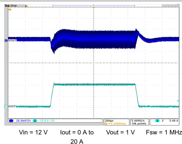
Figure 8-8. Load Transient
