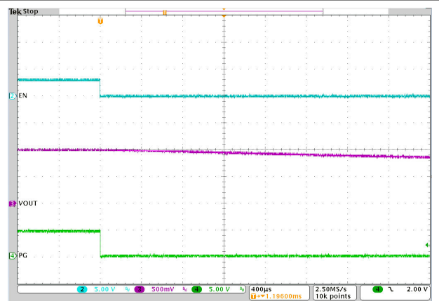
Figure 8-10. EN Shutdown
