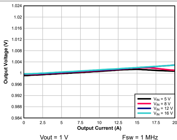
Figure 8-5. Load Regulation
