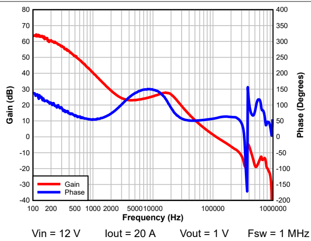
Figure 8-7. Bode Plot
