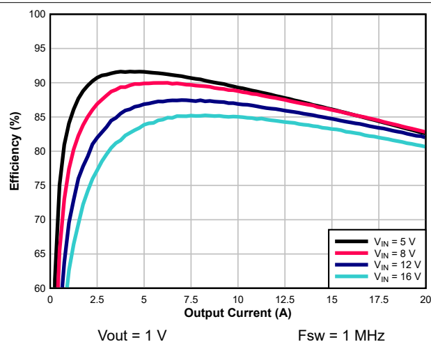
Figure 8-4. Efficiency Curves
