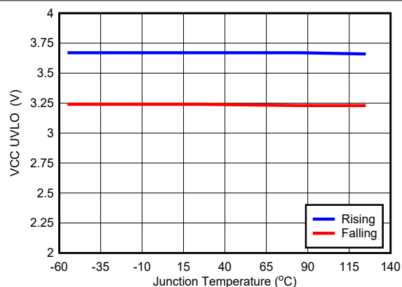
Figure 6-8. V_{CC} UVLO
