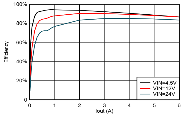
Figure 5-22. TPSM86638 Efficiency, V_{OUT} = 1.8V , F_{sw} = 800kHz
