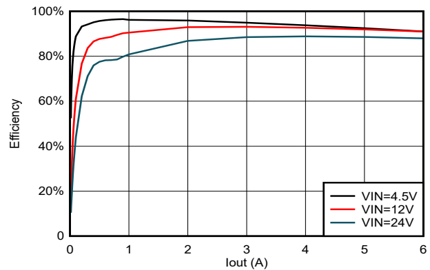
Figure 5-30. TPSM86638 Efficiency, V_{OUT} = 3.3V , F_{sw} = 1200kHz
