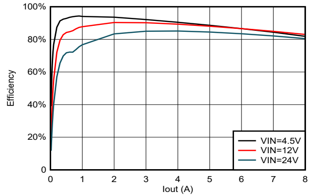
Figure 7-3. TPSM86838 Efficiency
