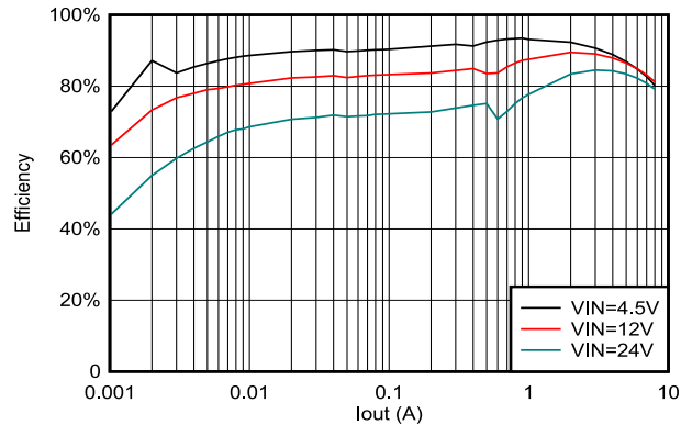
Figure 7-2. TPSM86837 Efficiency
