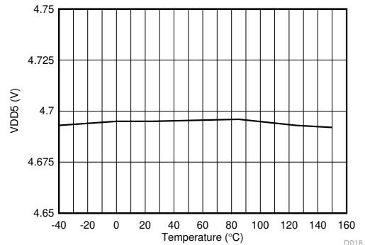
I_{VDD5} = 10mA V_{PIN} = V_{AVIN} = 12V Figure 5-8. VDD5 Voltage vs Junction Temperature
