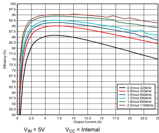
Figure 5-1. TPSM8S6B24S Efficiency vs Output Current
