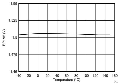
I_{BP1V5} = 2mA V_{PIN} = V_{AVIN} = 12V Figure 5-9. BP1V5 Voltage vs Junction Temperature
