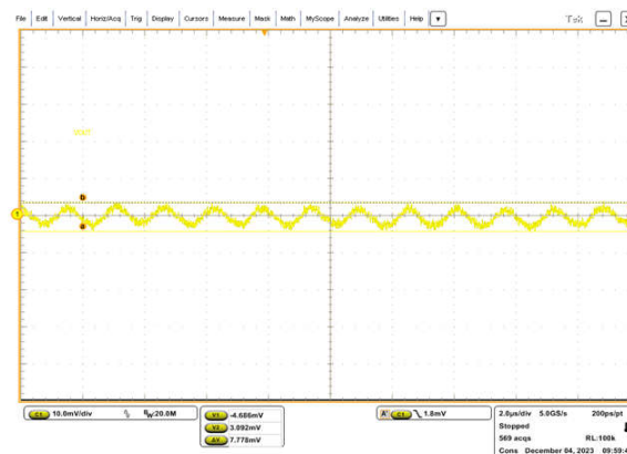
Figure 8-8. V_{OUT} Steady-State Ripple
