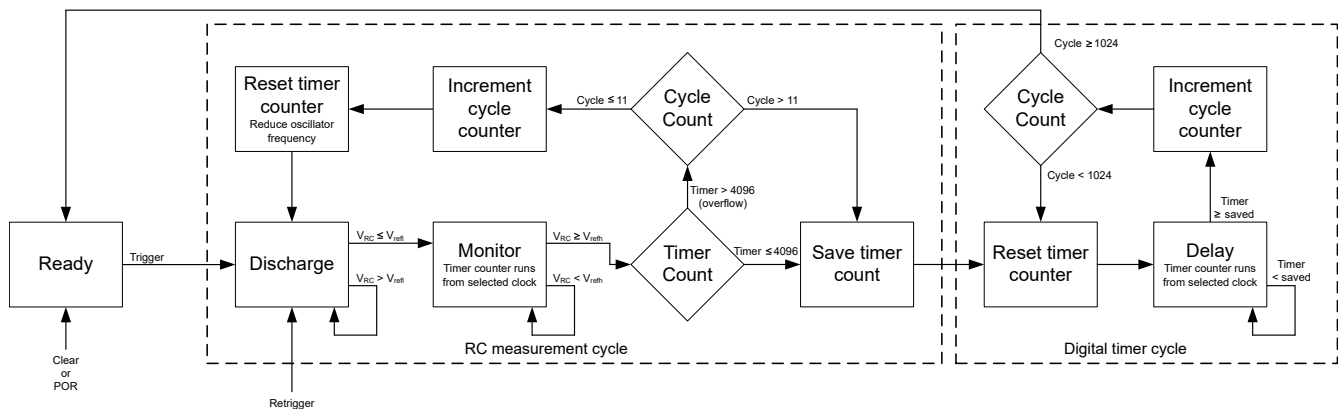
Figure 7-3. State Machine Diagram
