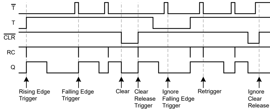
Figure 5-1. Timing Diagram
