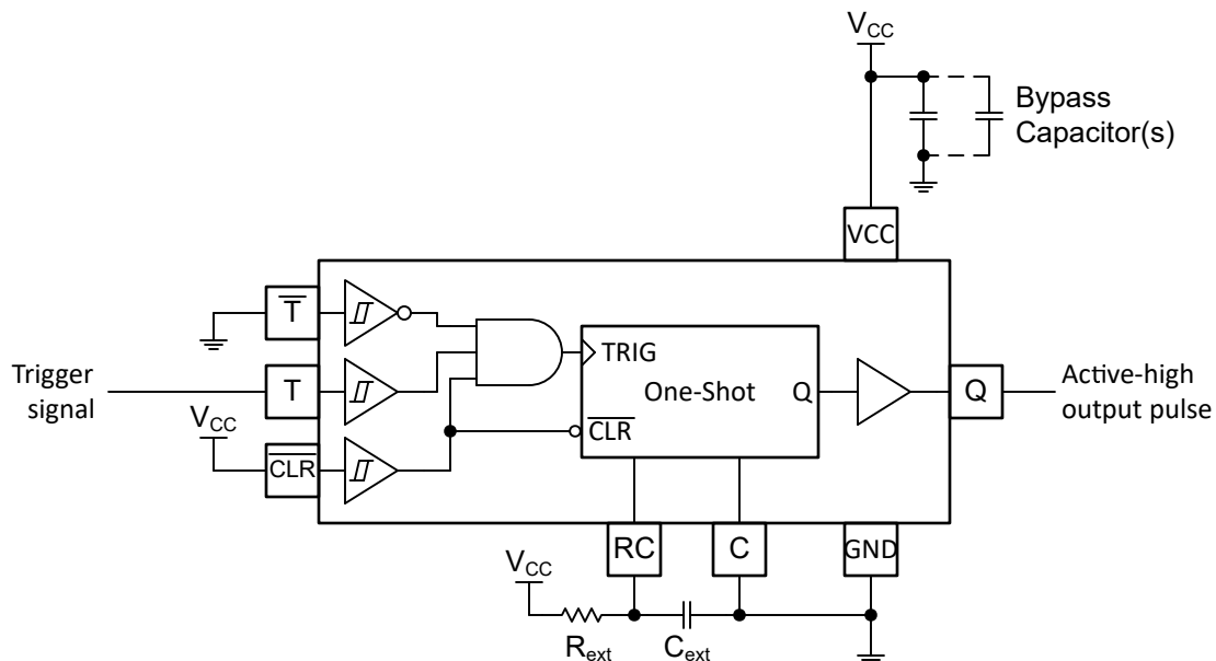
Figure 8-1. Pulse Generation Using the TPUL1G313-Q1
