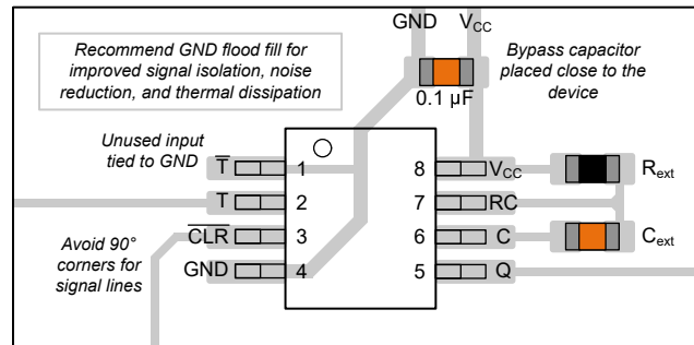
Figure 8-3. Layout Example
