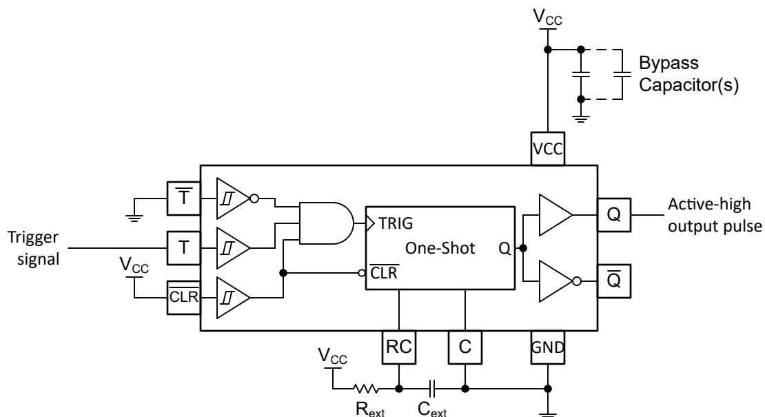
Figure 8-1. Pulse Generator Schematic Using the TPUL2G122x
