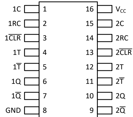
Figure 4-2. TPUL2G122A D and PW Package 16-Pin SOIC and TSSOP Top View
