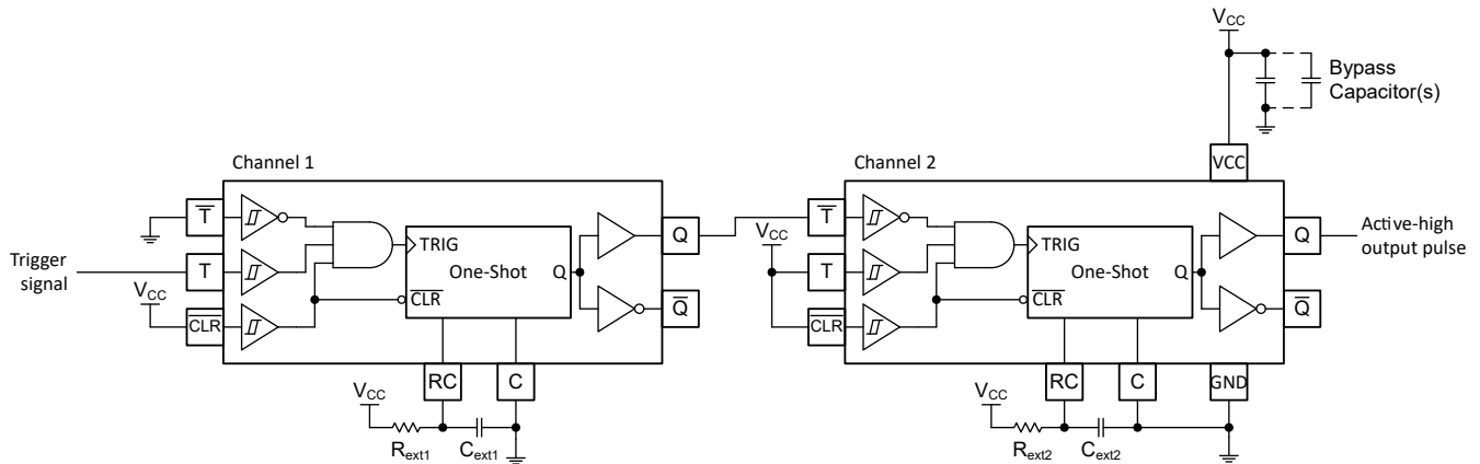
Figure 8-4. Delayed Pulse Generation Schematic Using the TPUL2G122x
