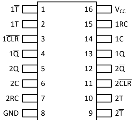
Figure 4-1. TPUL2G122 D and PW Package 16-Pin SOIC and TSSOP Top View
