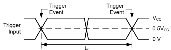
Figure 6-6. Voltage Waveforms, Retrigger Time
