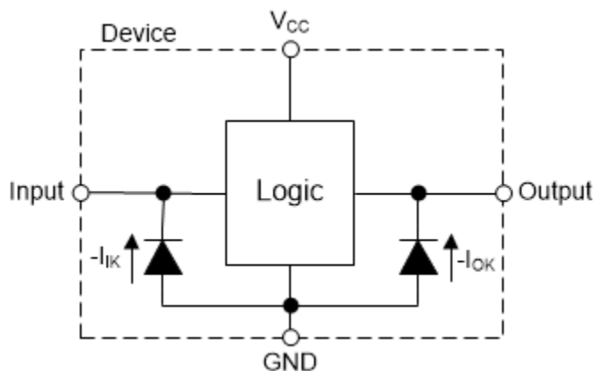
Figure 7-9. Electrical Placement of Clamping Diodes for Each Input and Output
