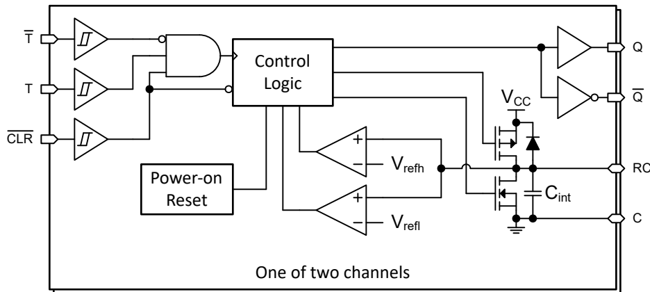
Figure 7-3. TPUL2T122-Q1
