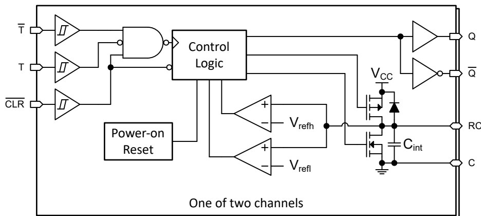
Figure 7-4. TPUL2T122A-Q1
