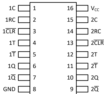
Figure 4-2. TPUL2T122A-Q1 D and PW Package 16-Pin SOIC and TSSOP Top View
