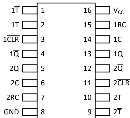
Figure 4-1. TPUL2T122-Q1 D and PW Package 16-Pin SOIC and TSSOP Top View
