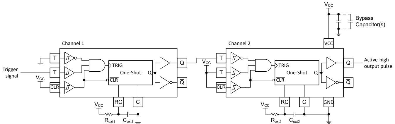
Figure 8-4. Delayed Pulse Generation Schematic Using the TPUL2T122x-Q1
