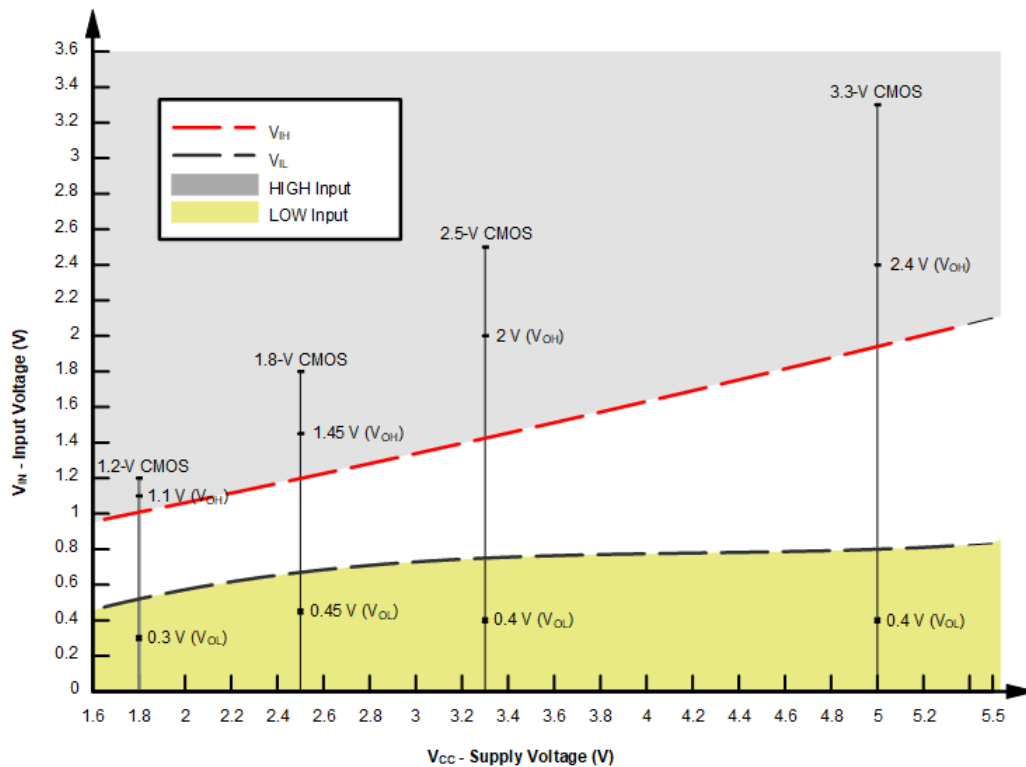
Figure 7-7. TPULxT Input Voltage Levels
