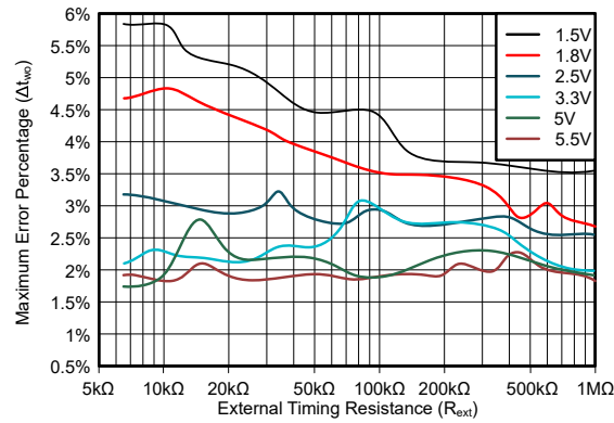
Figure 5-24. Maximum output pulse width error (absolute value) versus timing resistor values with C_{ext} = 1\text{nF}
