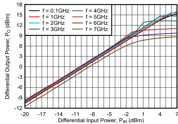
Figure 6-26. Differential Input vs Differential Output Power
