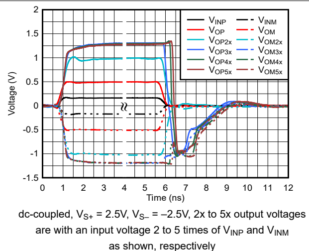
Figure 6-30. Overdrive Recovery Response
