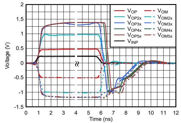
S2D, dc-coupled, V_{S+} = 2.5\text{V} , V_{S-} = -2.5\text{V} , 2x to 5x output voltages are with an input voltage 2 to 5 times that of V_{INP} as shown, respectively
