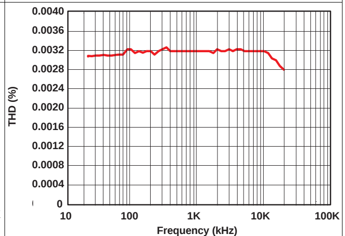
Figure 17. Total Harmonic Distortion vs Frequency ( R_L = 600 \Omega )
