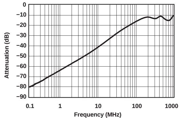
Figure 15. OFF Isolation vs Frequency ( V_{CC} = 3 V)
