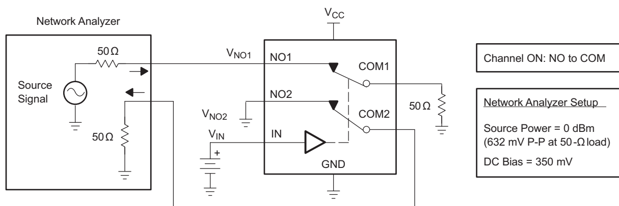
Figure 23. Crosstalk ( X_{TALK} )
