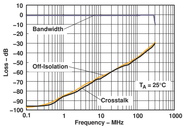
Figure 6-4. Frequency Response ( V_+ = 3\text{ V} )
