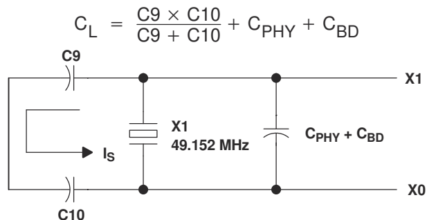
Figure 13-8. Load Capacitance for the TSB41BA3F-EP PHY
