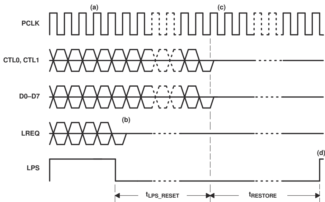
Figure 12-7. Interface Reset
