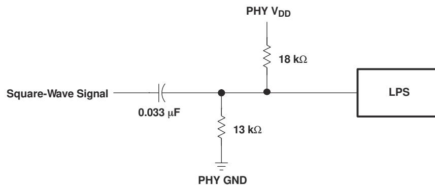
Figure 13-7. Isolated Circuit Connection For LPS
