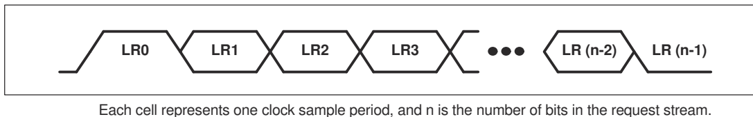
Figure 11-4. PINT (PHY Interrupt) Stream
