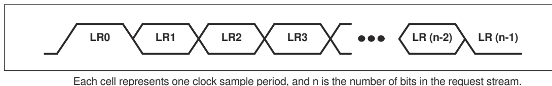
Figure 12-2. LREQ Request Stream
