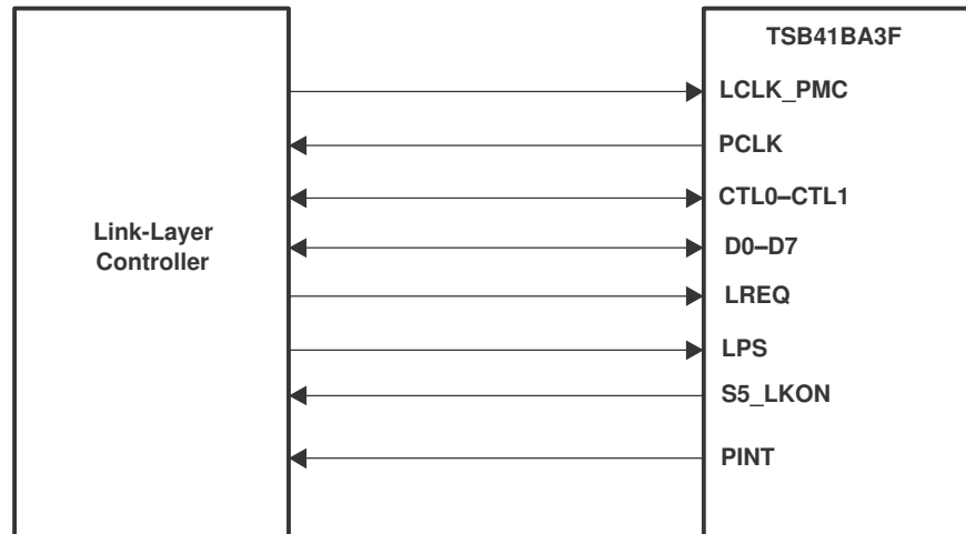
Figure 11-1. PHY-LLC Interface
