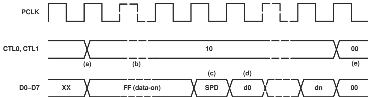
Figure 11-5. Normal Packet Reception Timing
