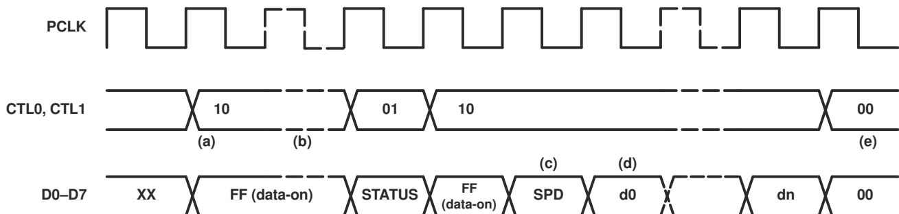
Figure 11-5. Normal Packet Reception Timing
