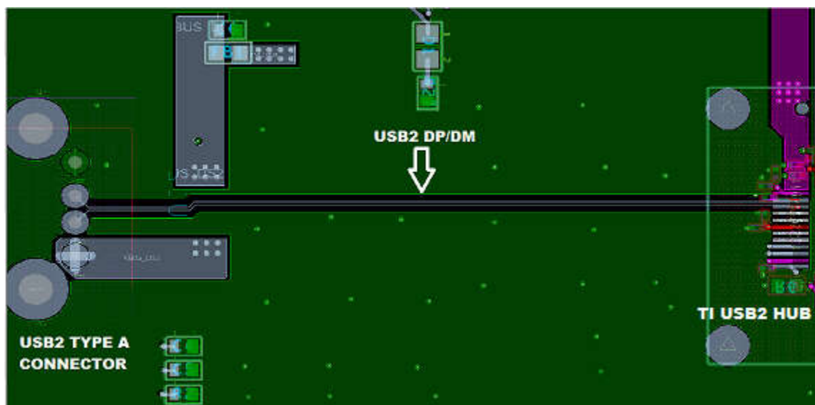
Figure 9-2. Downstream Port
