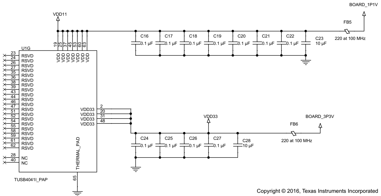
Figure 7-9. TUSB4041I Power Implementation
