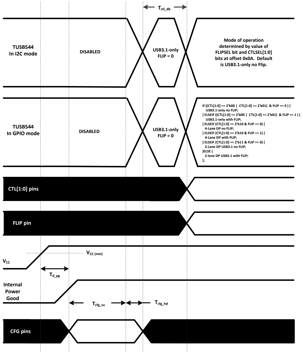
Figure 21. Power-Up Timing
