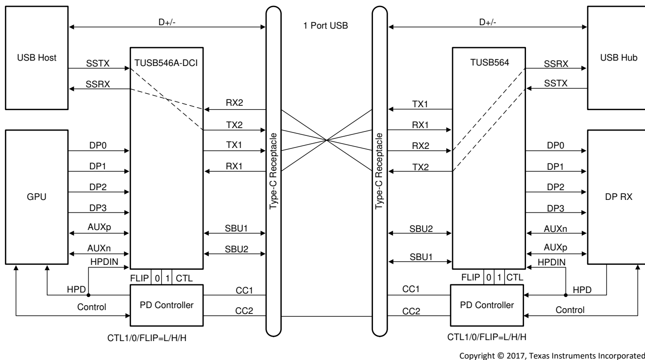
Figure 9-7. USB3.1 Only – With Flip (CTL1 = L, CTL0 = H, FLIP = H)
