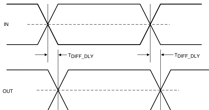
Figure 7-3. Propagation Delay
