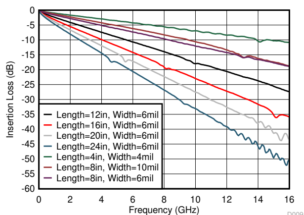
Figure 9-5. Insertion Loss of FR4 PCB Traces
