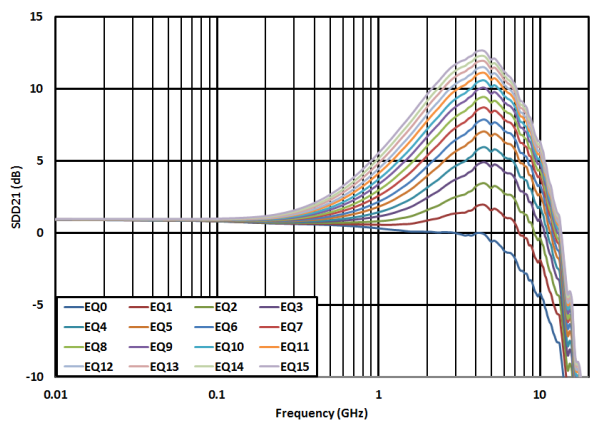
Figure 6-3. USB TX (UFP) EQ Settings Curves
