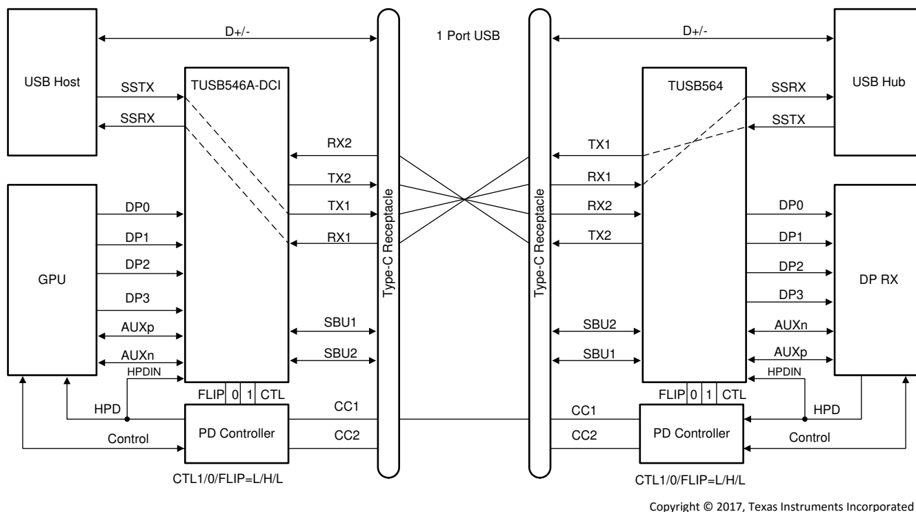
Figure 9-6. USB3.1 Only – No Flip (CTL1 = L, CTL0 = H, FLIP = L)
