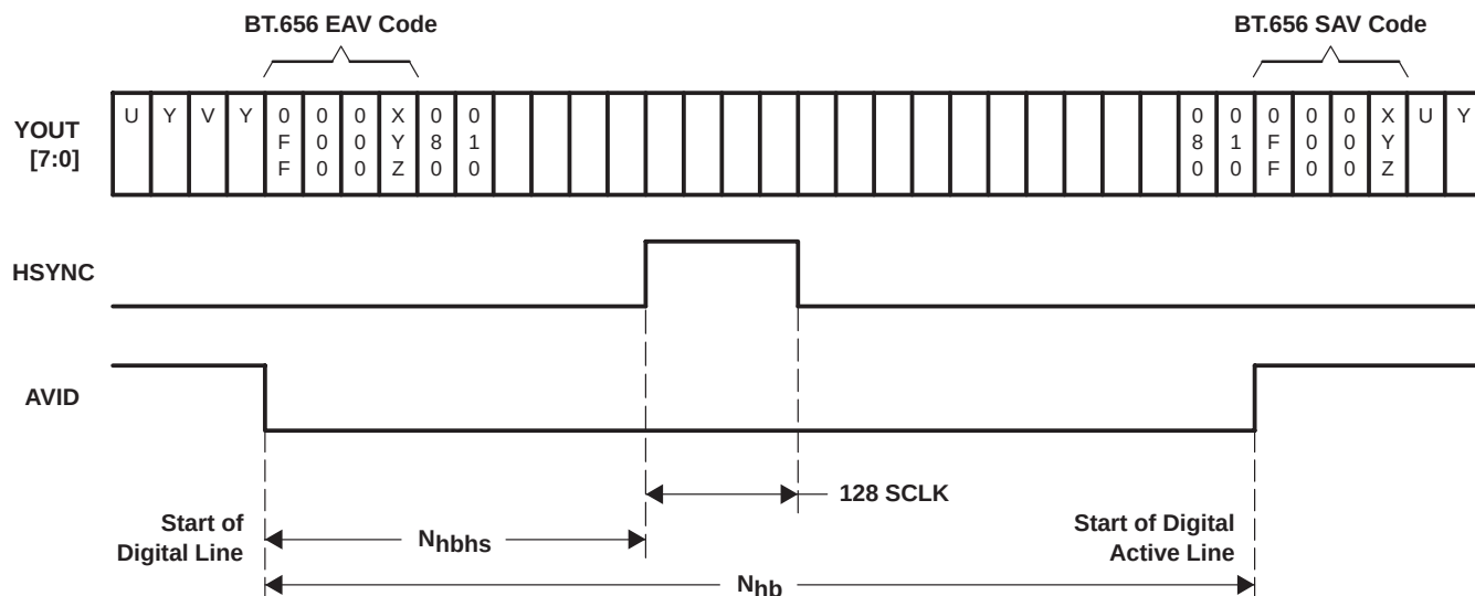
Figure 3–15. Horizontal Sync
