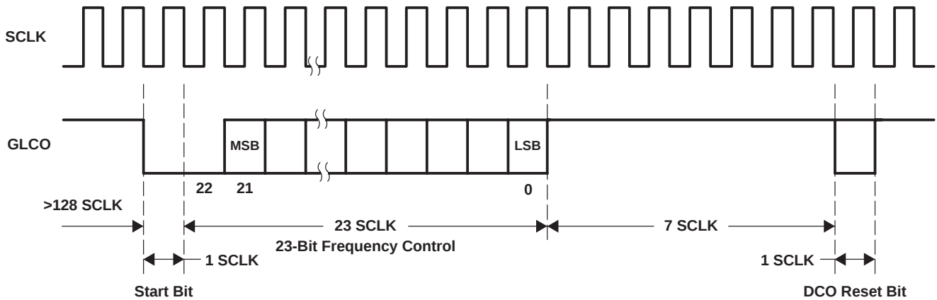
Figure 2–6. GLCO Timing
