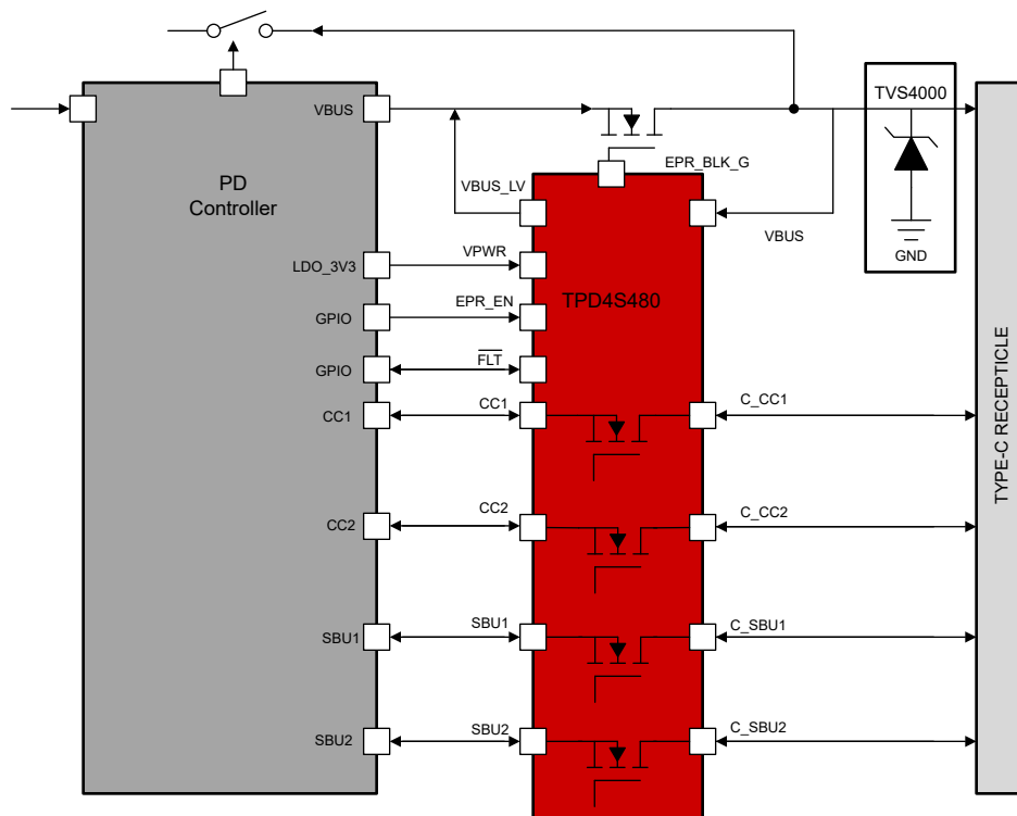
Figure 9-1. TVS4000 Application Schematic
