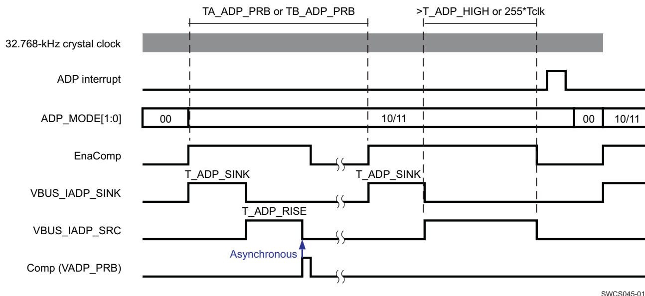
Figure 20. ADP Probing Timing Diagram
