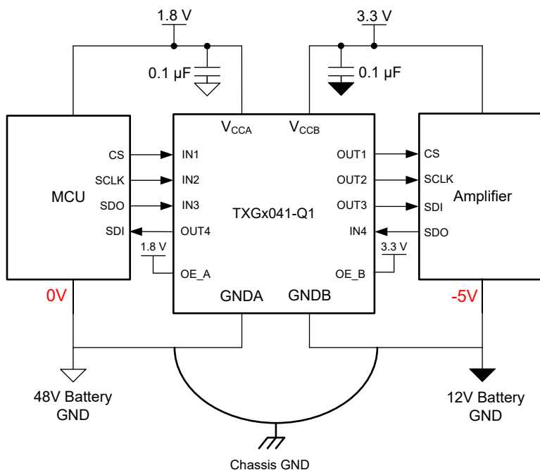
Figure 8-1. TXG1041-Q1 in Automotive
