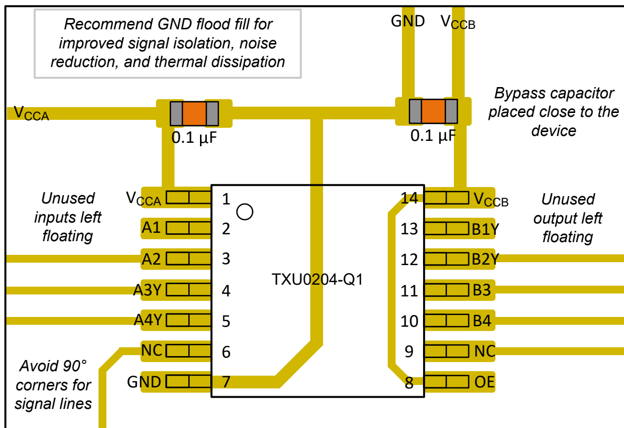
Figure 9-3. Layout Example – TXU0204-Q1
