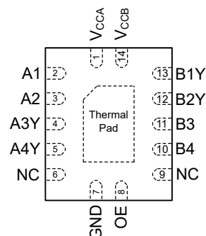
Figure 5-2. WBQA Package, 14-Pin VQFN Transparent (Top View)
