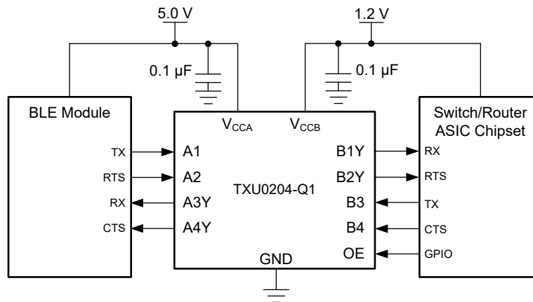
Figure 9-1. TXU0204-Q1 UART Interface Application
