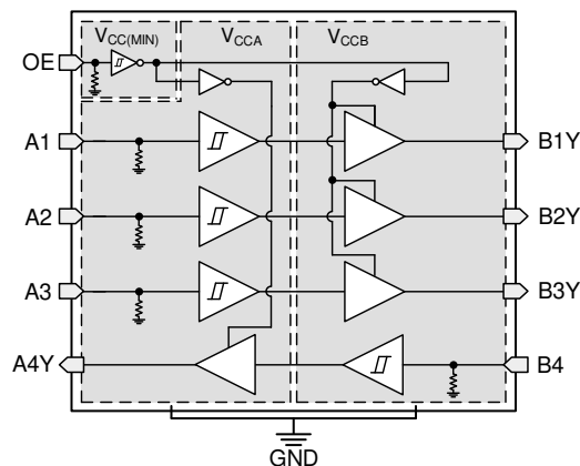
Figure 4-2. TXU0304-Q1 Functional Block Diagram
