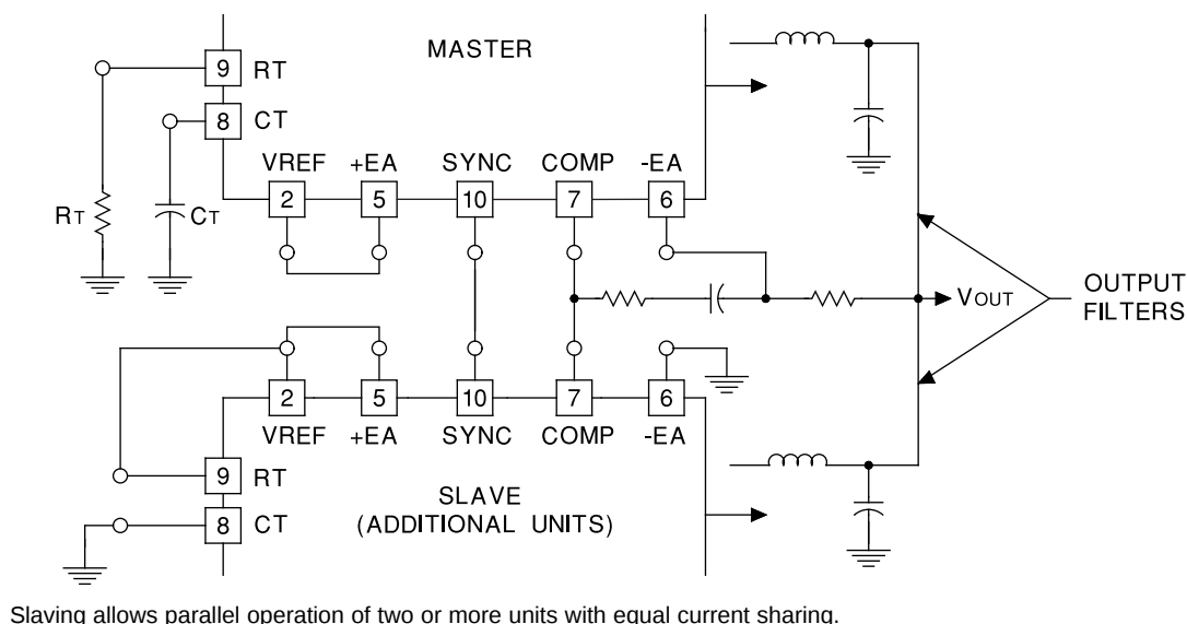
Figure 12. Parallel Operation
