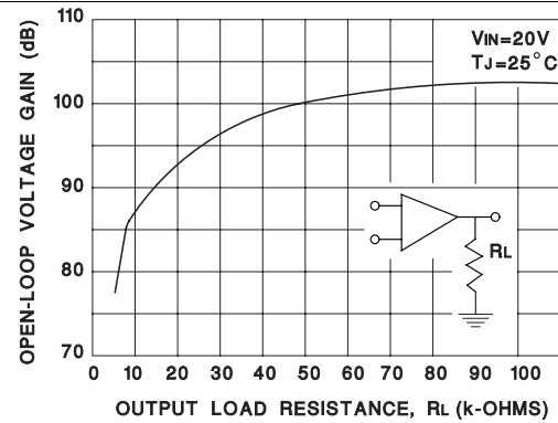
Figure 2. Error amplifier Open-Logic DC Gain vs Load Resistance
