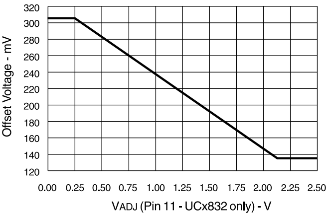
Current Sense Amplifier Offset Voltage vs V ADJ
