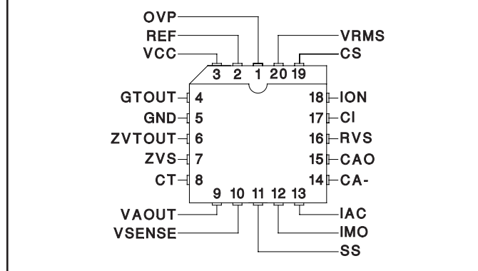
PLCC-20 & LCC-20 (Top View) Q or L Package
