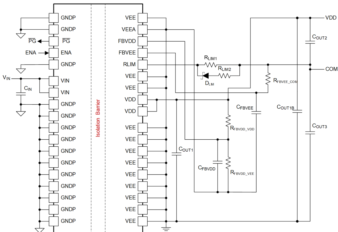
Figure 12-9. Dual output application schematic configured for V_{COM\_VEE} regulation = 2.5V
