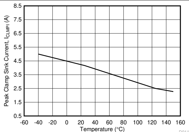
Figure 5-22. I CLMPI Miller Clamp Sink Current vs. Temperature
