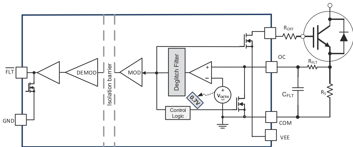
Figure 8-10. Overcurrent and Short Circuit Protection Based on Shunt Resistor
