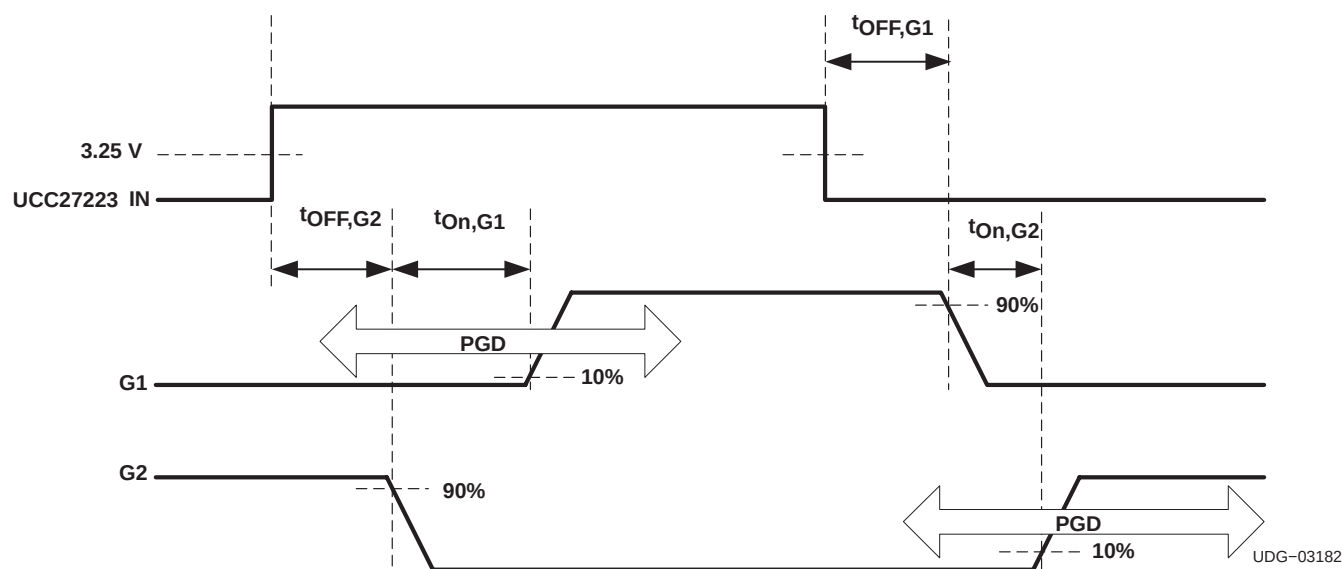
Figure 2. Predictive Gate Drive Timing Diagram
