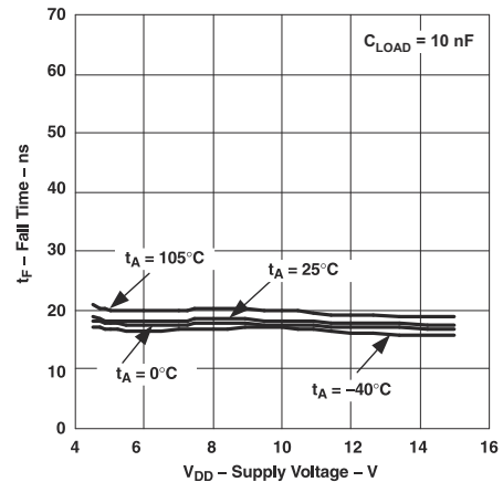
Figure 7-8. Fall Time vs Supply Voltage
