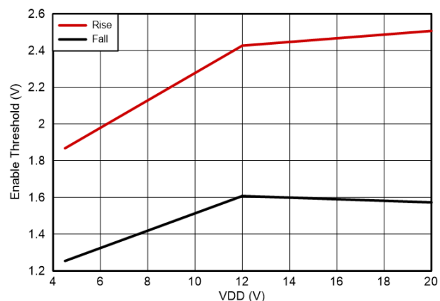
Figure 6-8. Enable Threshold
