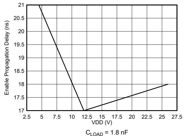
Figure 6-20. Enable to Output Rising Propagation Delay
