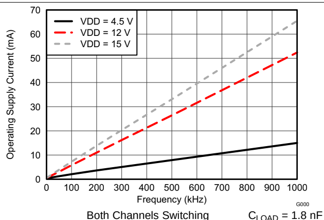
Figure 15. Operating Supply Current vs Frequency
