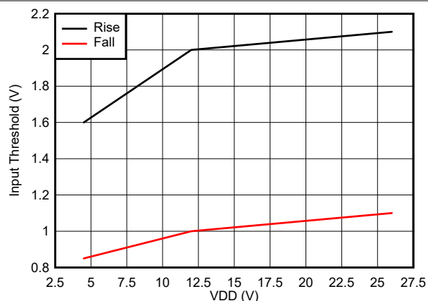
Figure 5-8. Input Thresholds
