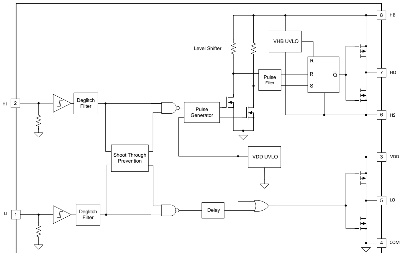
Figure 29. UCC27712-Q1 Block Diagram
