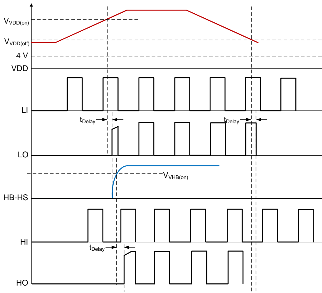
Figure 30. Power-Up Driver
