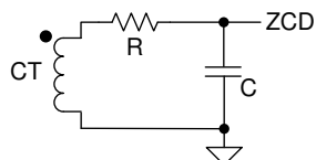
Figure 18. Simple RC Delay Circuit
