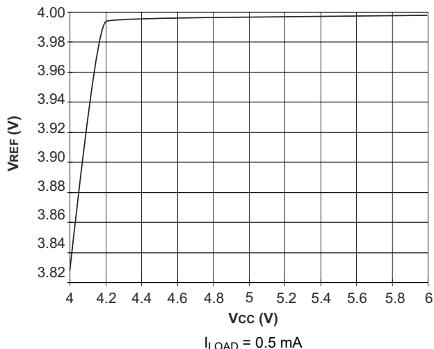
Figure 6-2. UCC3813-[3,5]: V_{REF} vs V_{CC}
