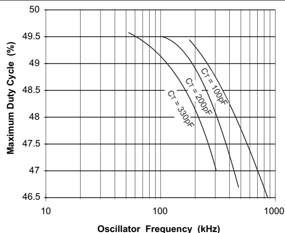
Figure 6-6. UCC3813-[1,4,5]: Maximum Duty Cycle vs Oscillator Frequency
