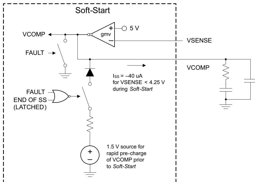
Figure 23. Soft Start
