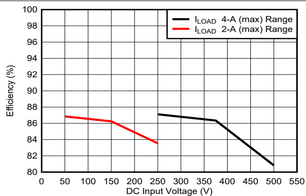
Figure 8-5. 10%-Load Efficiency vs. DC Input Voltage
