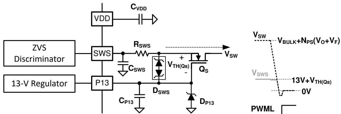
Figure 7-6. ZVS Sensing by Reusing the VDD Startup Circuit
