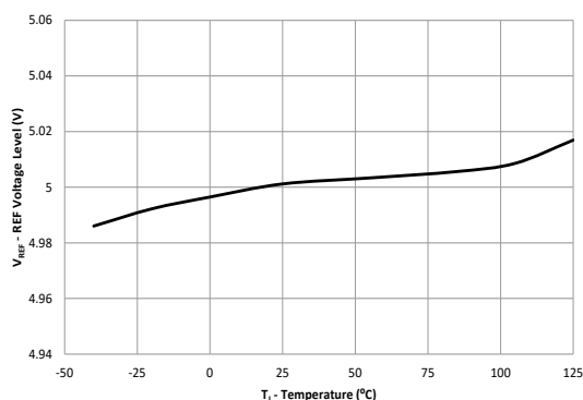
Figure 6-9. REF Voltage vs. Temperature
