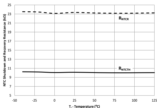
Figure 6-11. FLT OTP Thresholds vs. Junction Temperature
