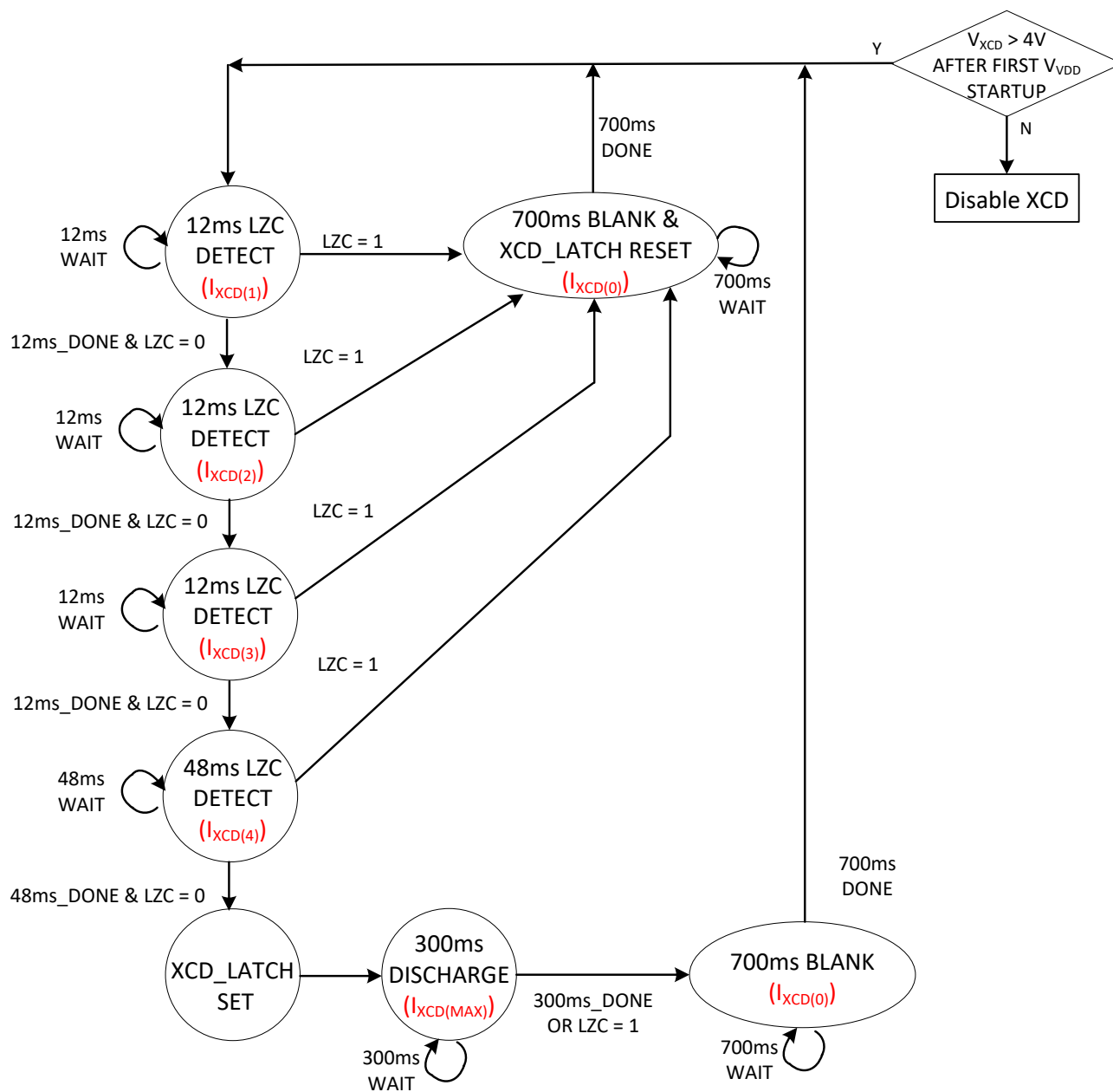
Figure 7-20. The State Diagram of the XCD-pin Function
