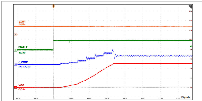
Figure 8-2. Start-Up with EN/FLT From Low to High: VINP = 5.0V, VCC = 5.0V, 18Ω Load
