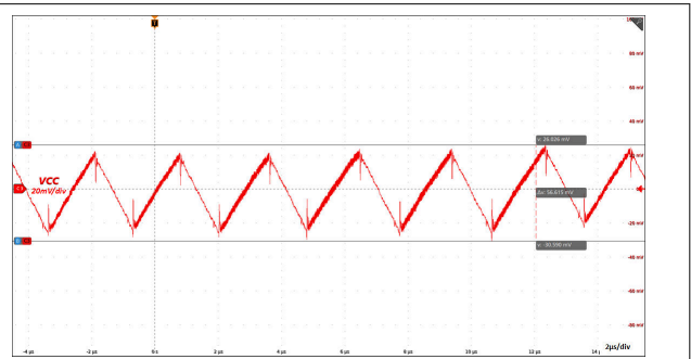
Figure 8-3. Steady State Output Voltage Ripple: VINP = 5.0V, VCC = 5.0V, 300mA Load
