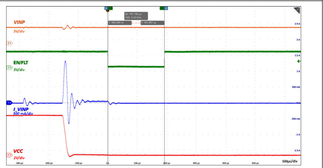
Figure 8-5. Output Short Circuit Operation: VINP = 5.0V
