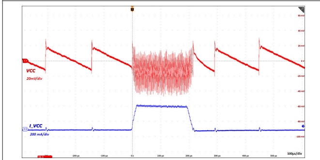
Figure 8-4. Load Transient: VINP = 5.0V, VCC = 5.0V, C OUT2 = 22μF, I VCC = 0mA - 300mA - 0mA
