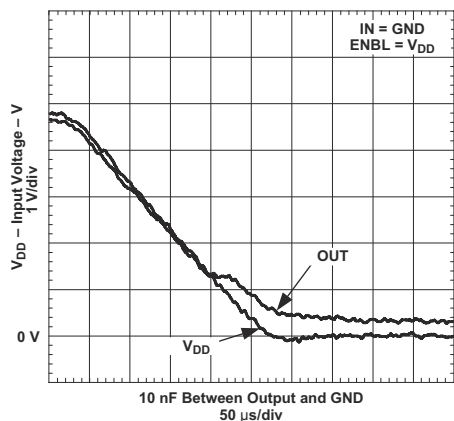
Figure 7-20. Output Behavior vs V_{DD} (UCC37321)
