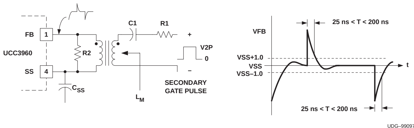
Figure 3. Pulse Edge Transmission (PET) Circuit
