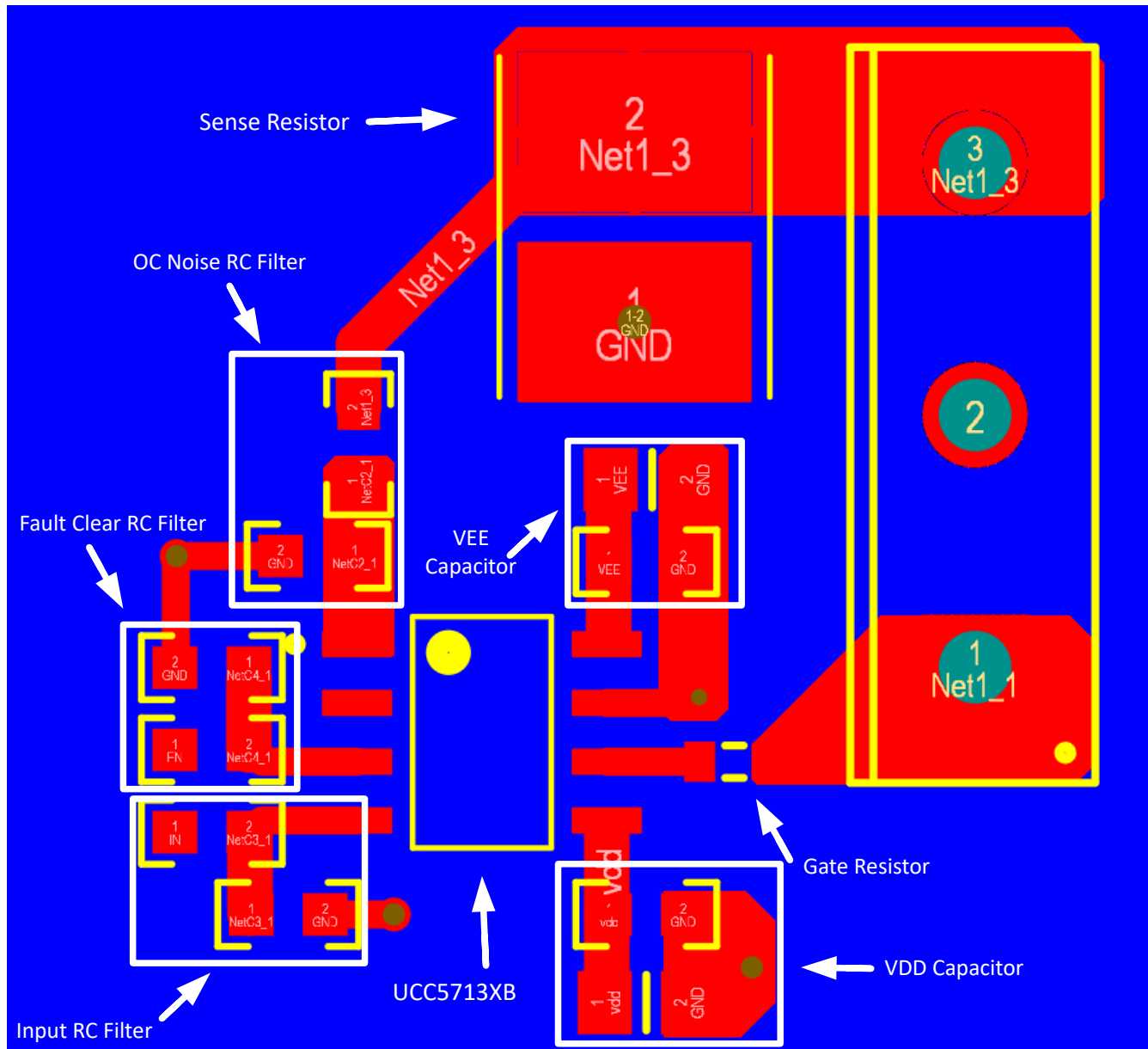
Figure 7-5. Layout Example: UCC5713x-Q1D
