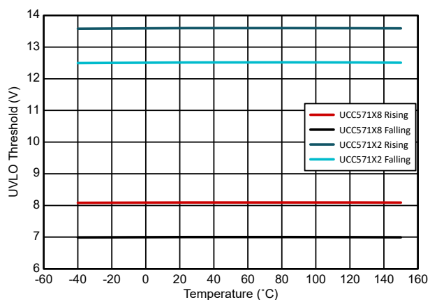
Figure 5-6. UVLO Threshold
