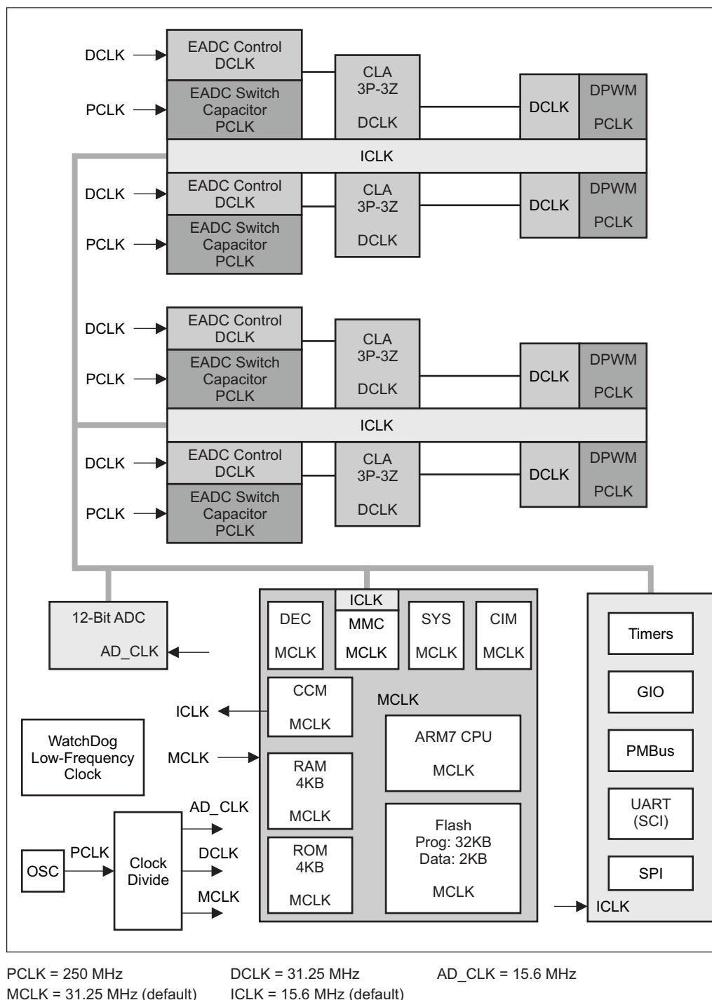
Figure 3. UCD30xx Clock Domains
