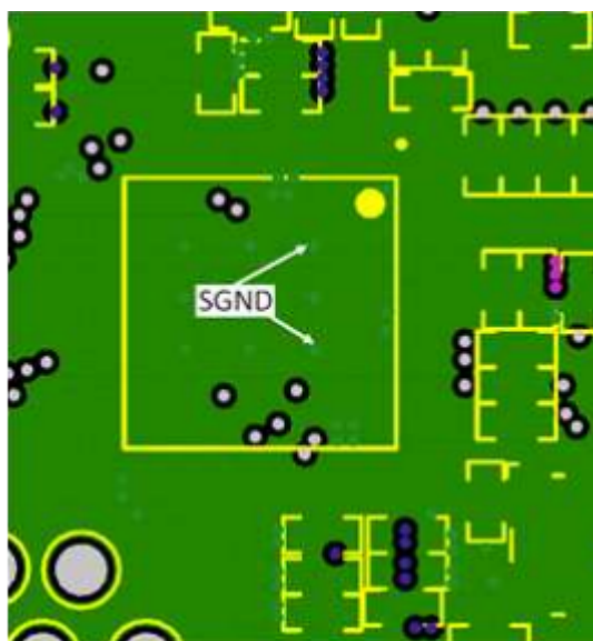
Figure 50. Layout Example
