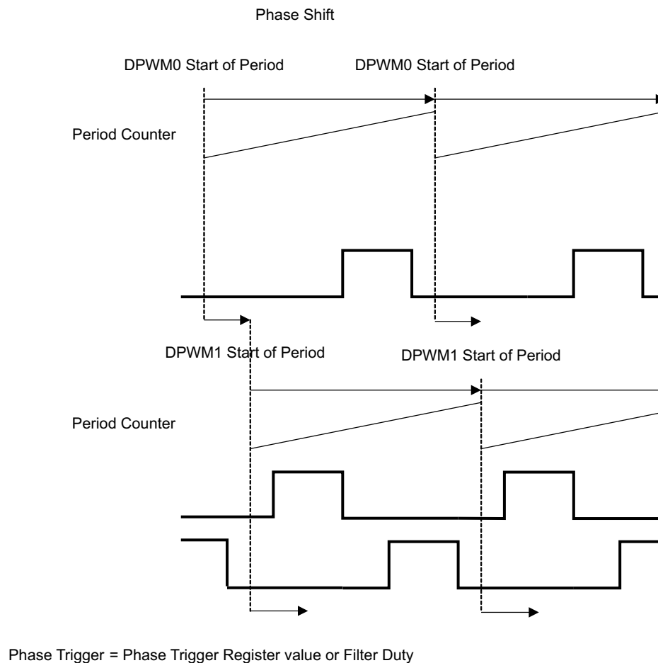
Figure 30. Phase Shifting
